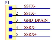
Header 5X1 _2.54mm
