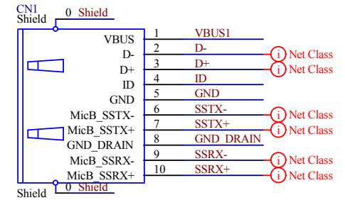
Micro USB3.0 Type B Female
